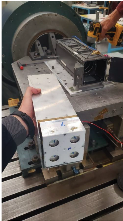
Figure 9. Vibration Testing of the PATCOOL CubeSat Prototype
