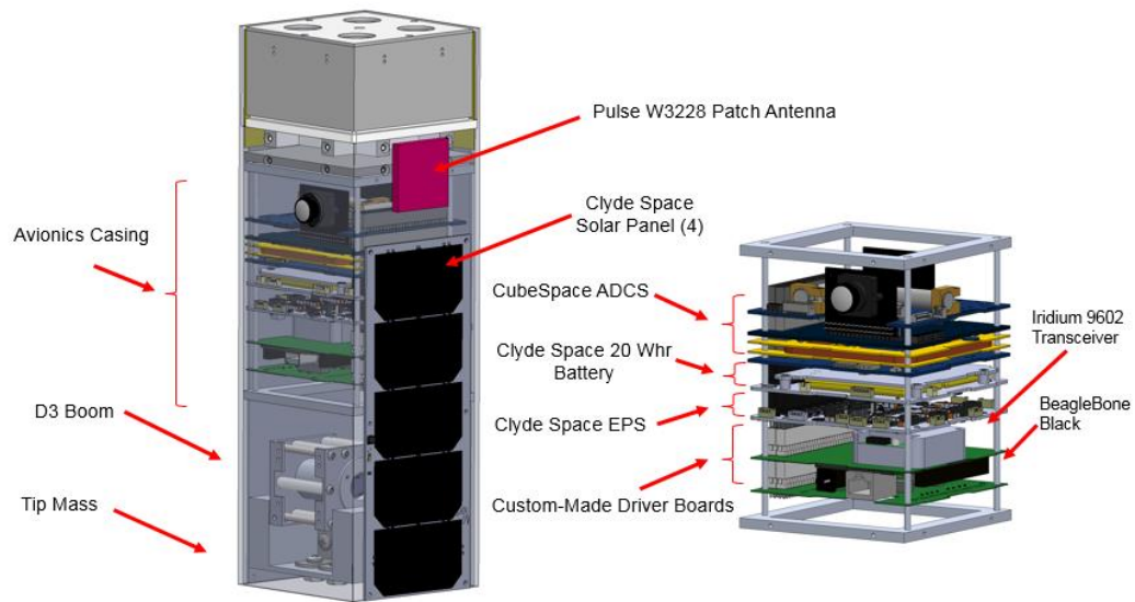
Figure 3. Avionics Components and Interfacing
