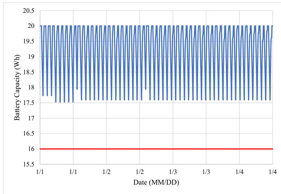
Figure 4. COTS ADCS Worst-Case Battery Capacity, RAAN = 0 deg
