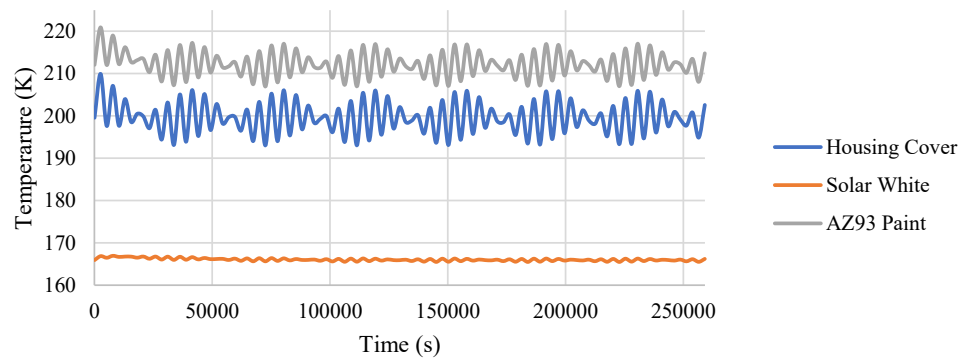
Figure 8. PATCOOL Temperature Response over Time
