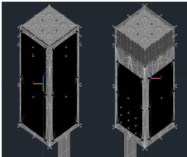
Figure 6. Simplified PATCOOL CubeSat Model for Thermal Analysis
