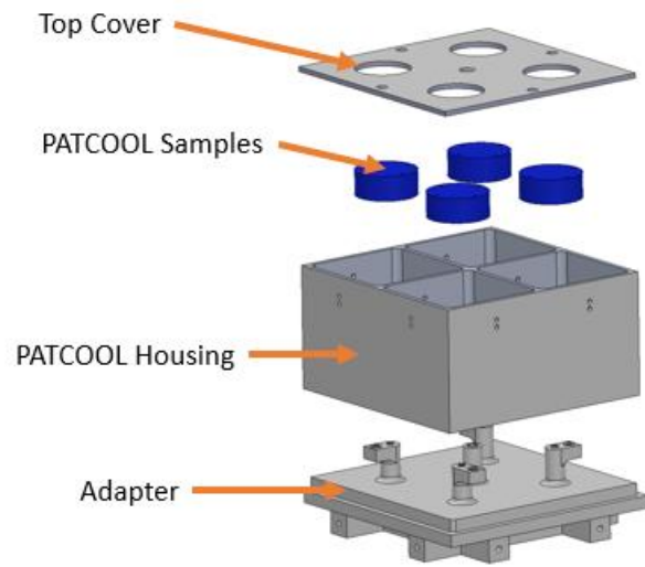
Figure 1. PATCOOL Payload and CubeSat Adapter
