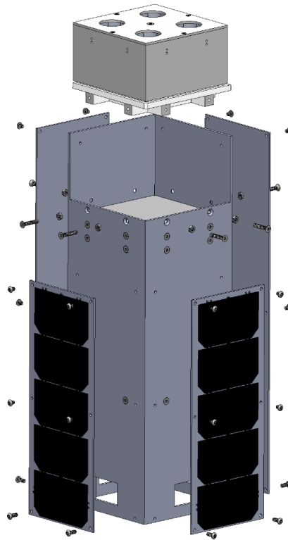
Figure 2. PATCOOL Structure and Payload with Solar Panels
