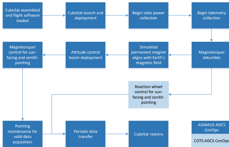
Figure 10. PATCOOL Mission Concept of Operations
